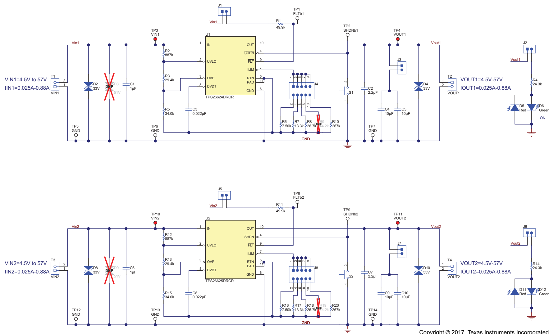
Figure 1. TPS26624-25EVM Schematic
